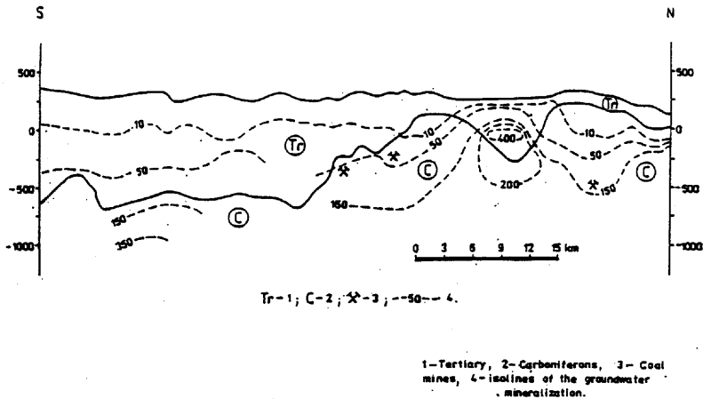
Figure 4. Hydrochemical cross-section (1) Tertiary (2) Carboniferous (3) Coal Mines and (4) Isolines of ground water mineralisation
