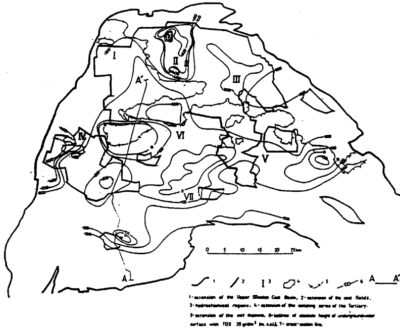
Figure 3. Sketch-map of the surface of brines (USCB) with TDS 35g/dm 3
